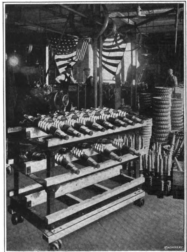
Fig. 4—Worm drives for rear axle transmissions are made in large quantities at the plant of the Timken-Detroit Axle Co. Of course, these worms and the worm-shaft bearings, etc., are carefully machined and precautions must be taken to prevent damage through one worm striking another. This is accomplished by the use of special trucks with "cradles" in which the worms are held without danger of damage
